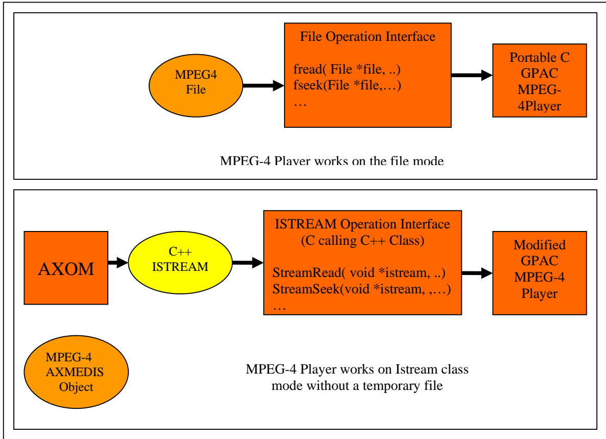
Figure: MPEG-4 Player accesses MPEG4-resource from an AXMEDIS object using an ISTREAM operation interface without a temporary file
