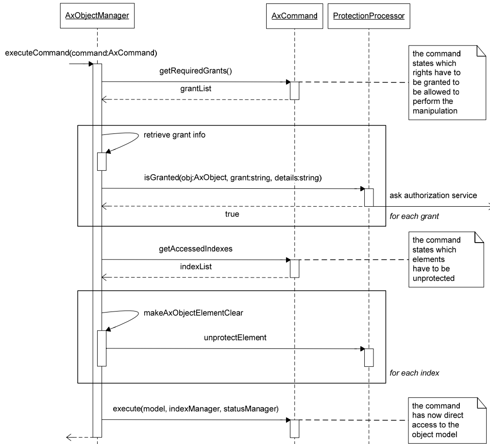
Sequence diagram of a command execution
