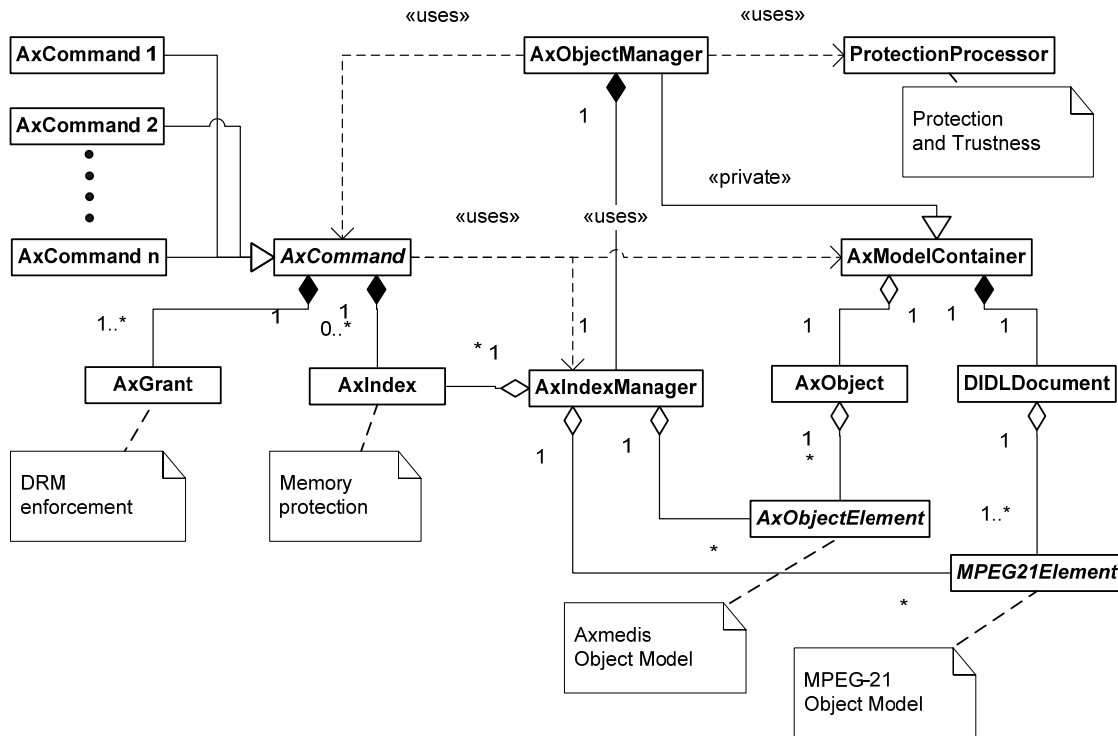
AXOM class hierarchy
