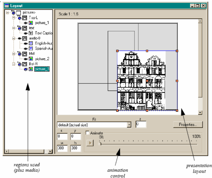
Figure 8 - Layout of the GRiNS editor
