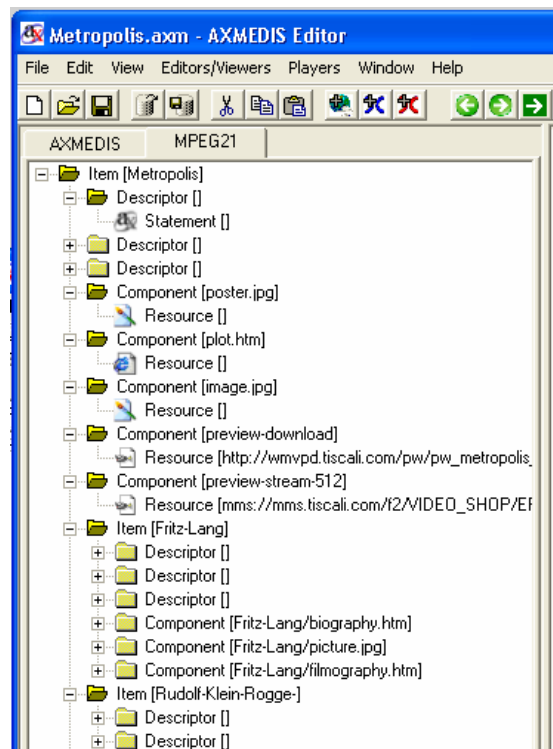
Figure 7 - Example of MPEG-21 hierarchy
