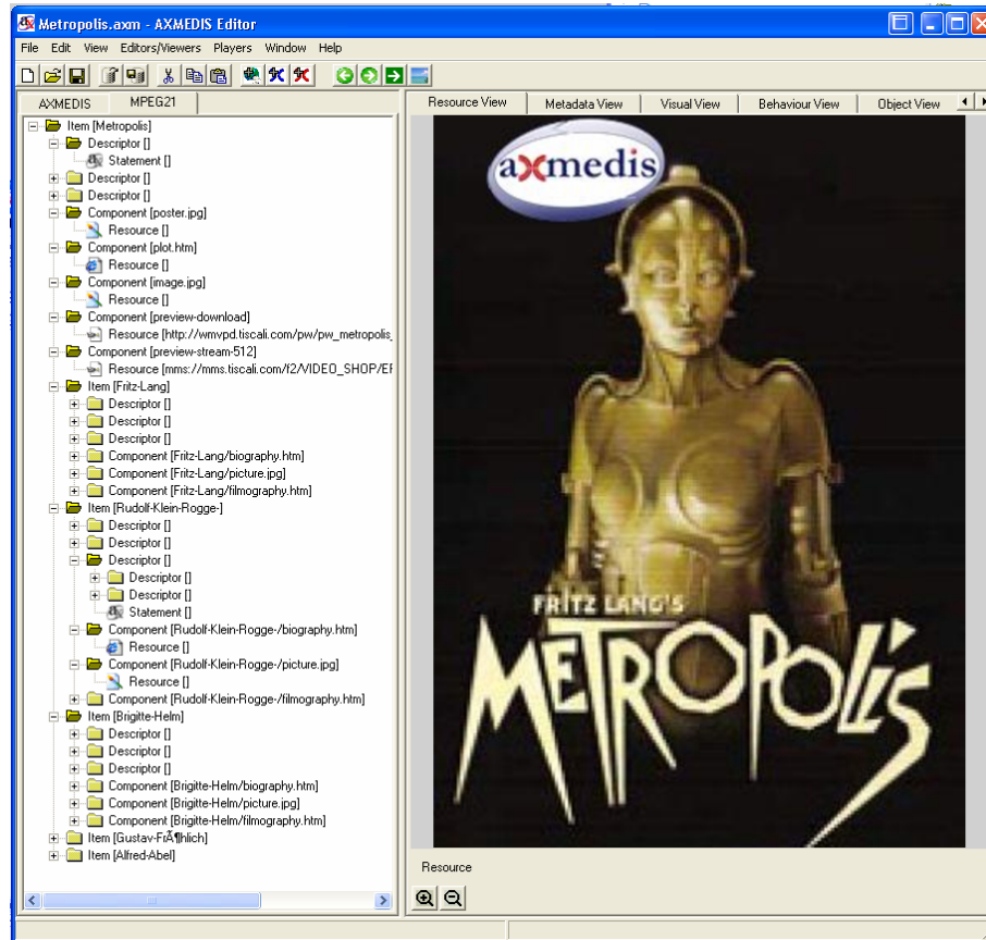
Views of the AXMEDIS Editor for the same object shown in the above Figure by the player. Please note that the editor is capable of showing the object as an AXMEDIS hierarchy, or an MPEG-21 hierarchy. In this case an MPEG-21 hierarchy is shown.
