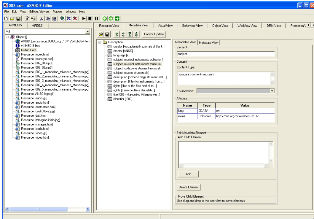
Figure 10 – AXMEDIS Editor with the Metadata View Editor panel to edit the Dublin Core.
