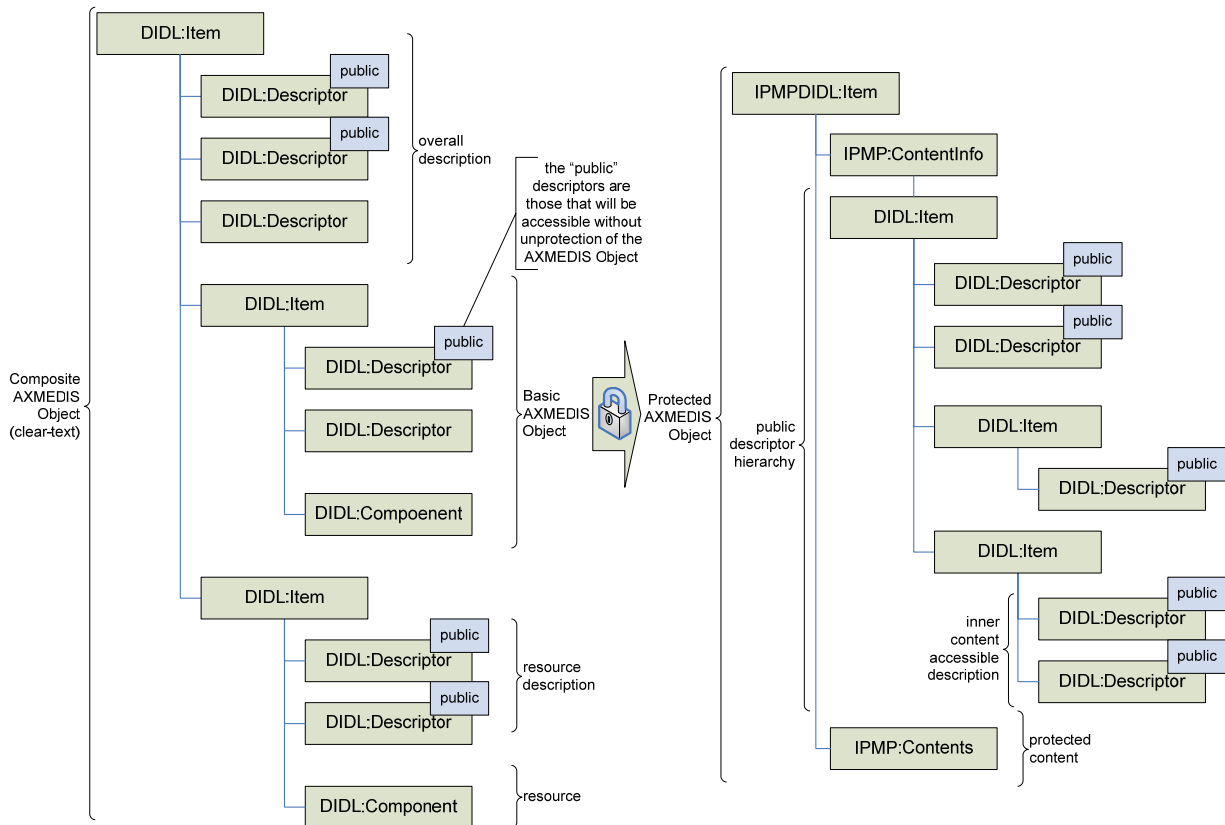
AXMEDIS Object after protection in terms of MPEG-21 elements
