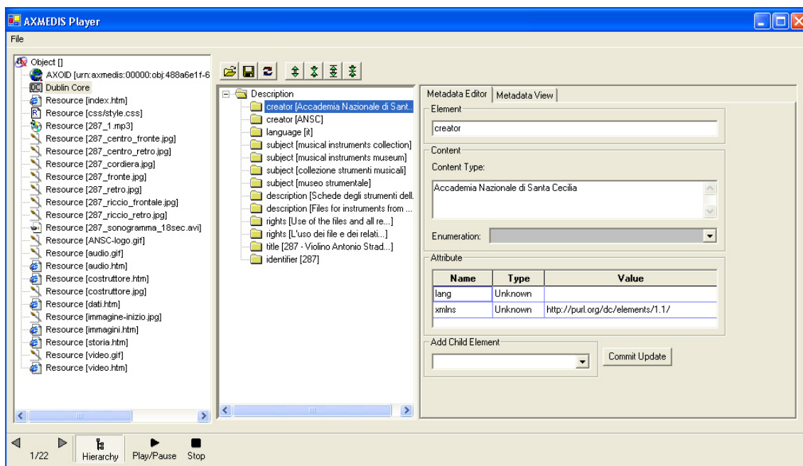
Figure 163 – AXEDIS Dublin Core metadata view
