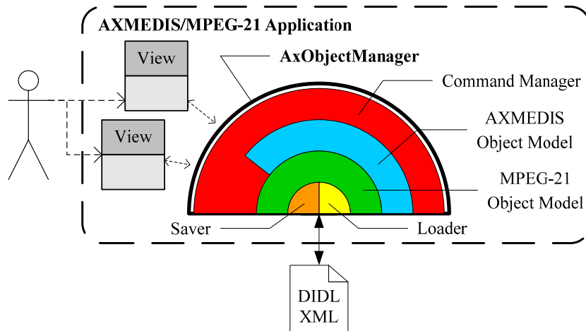
AXMEDIS Object Manager (AXOM) layers
