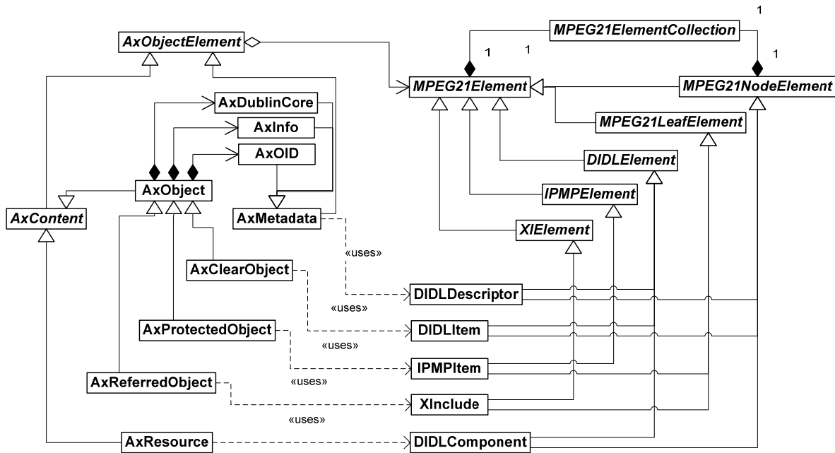
AXMEDIS and MPEG-21 Object Models relationships
